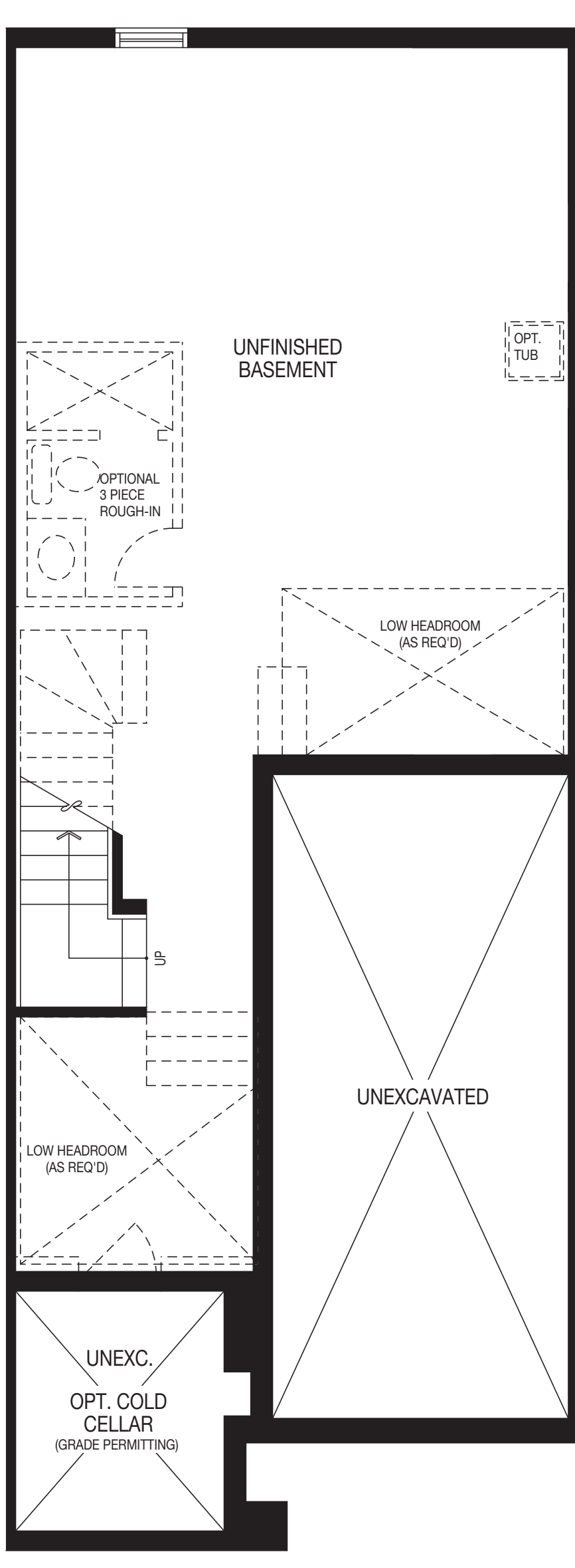
Basement ELEVATION A/B
