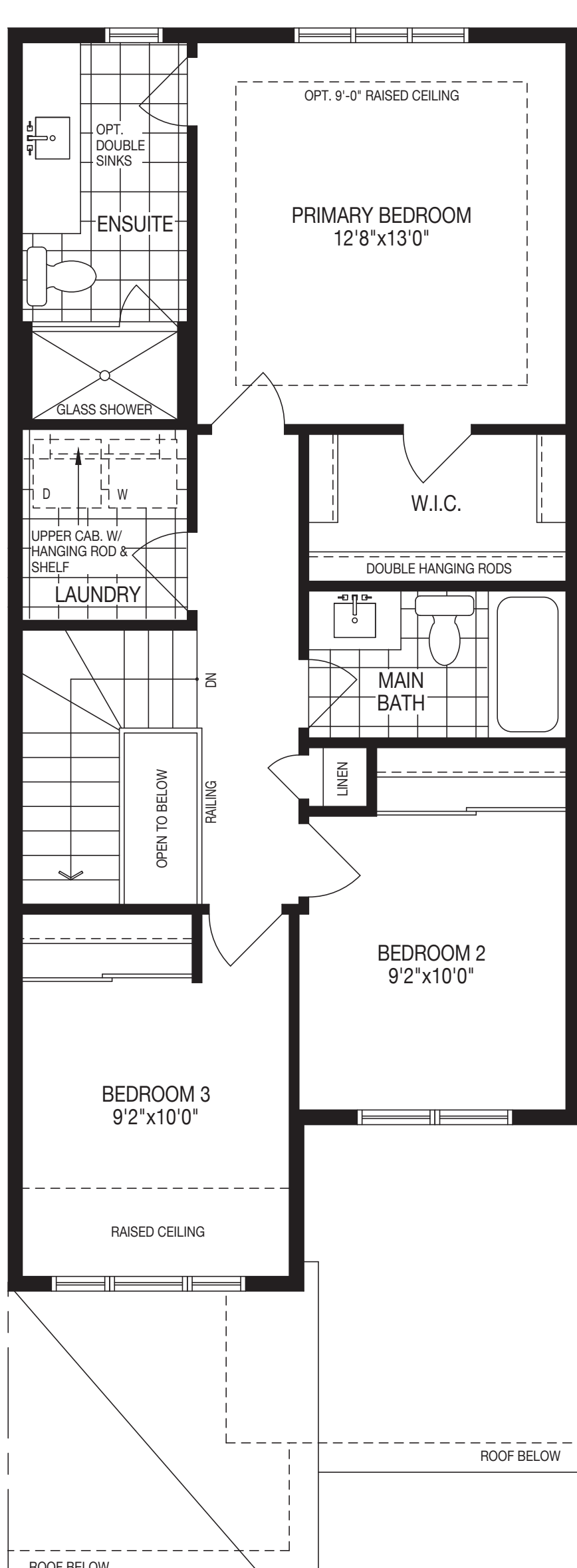
Second Floor ELEVATION A
