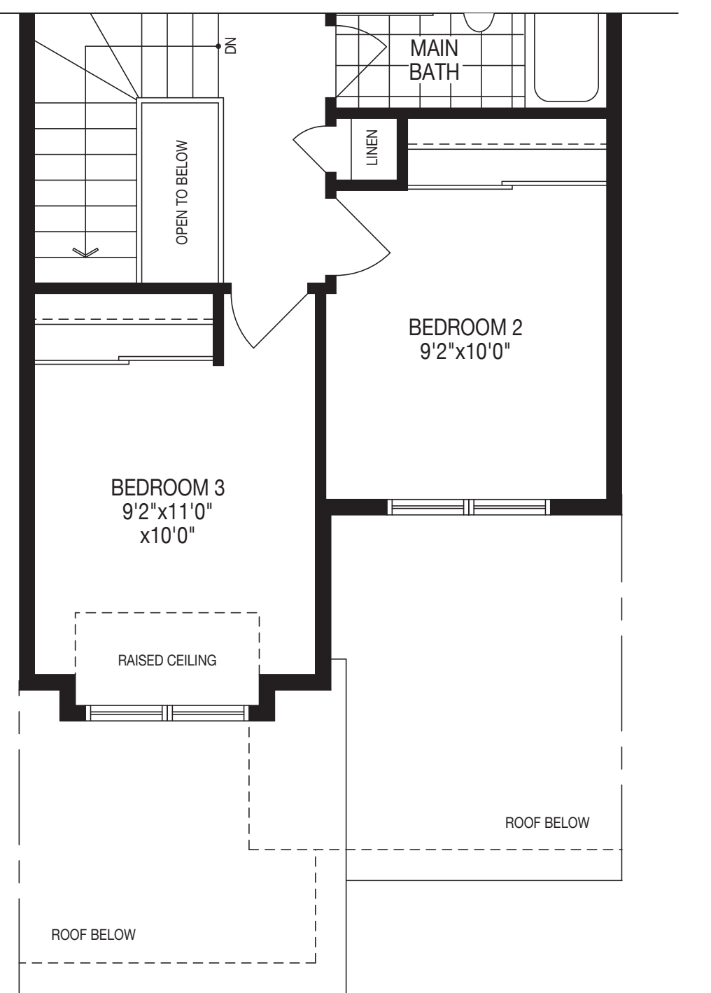
Second Floor ELEVATION B
