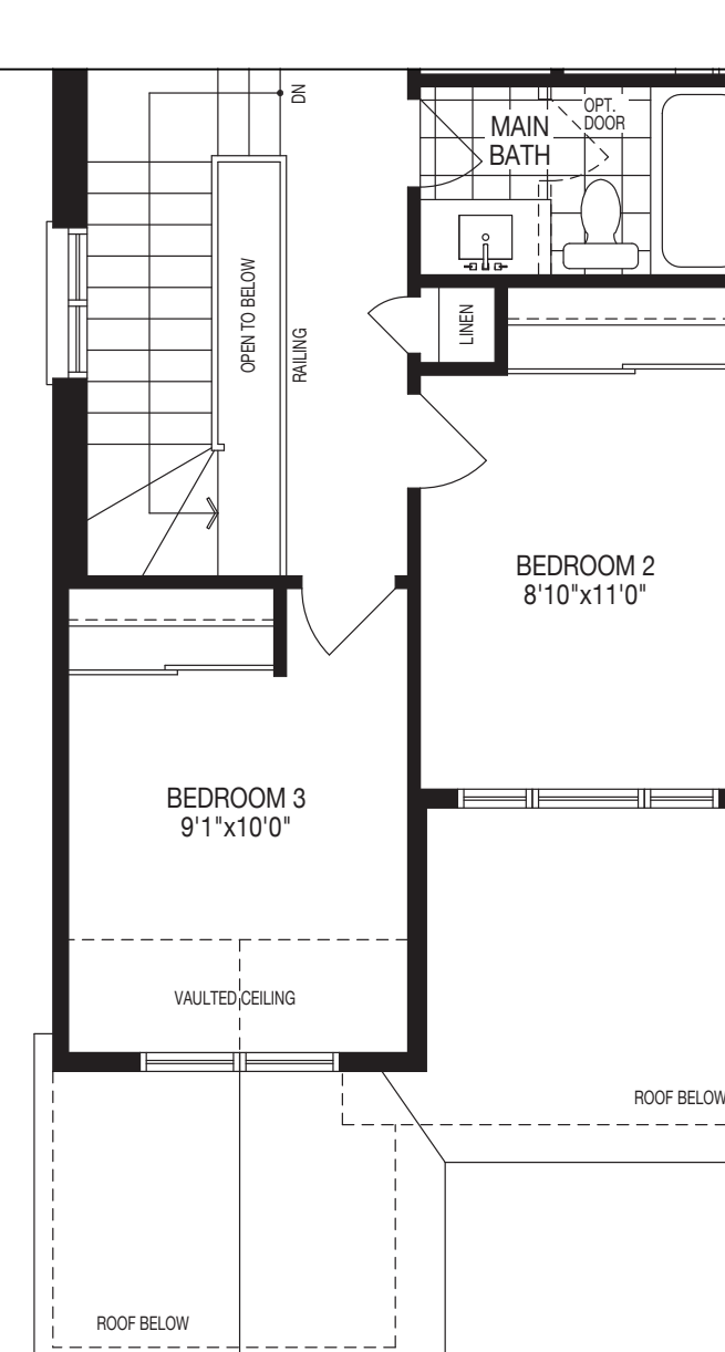
Second Floor ELEVATION B - OPT. 4 BEDROOM
