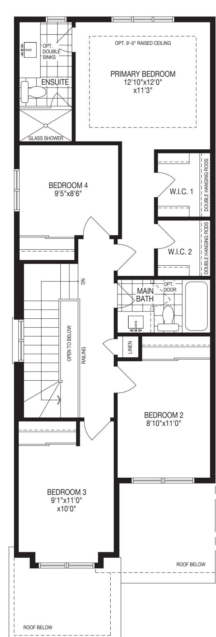
Second Floor ELEVATION A - OPT. 4 BEDROOM
