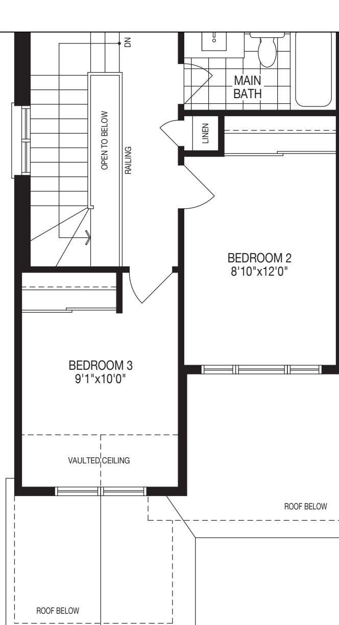
Second Floor ELEVATION B
