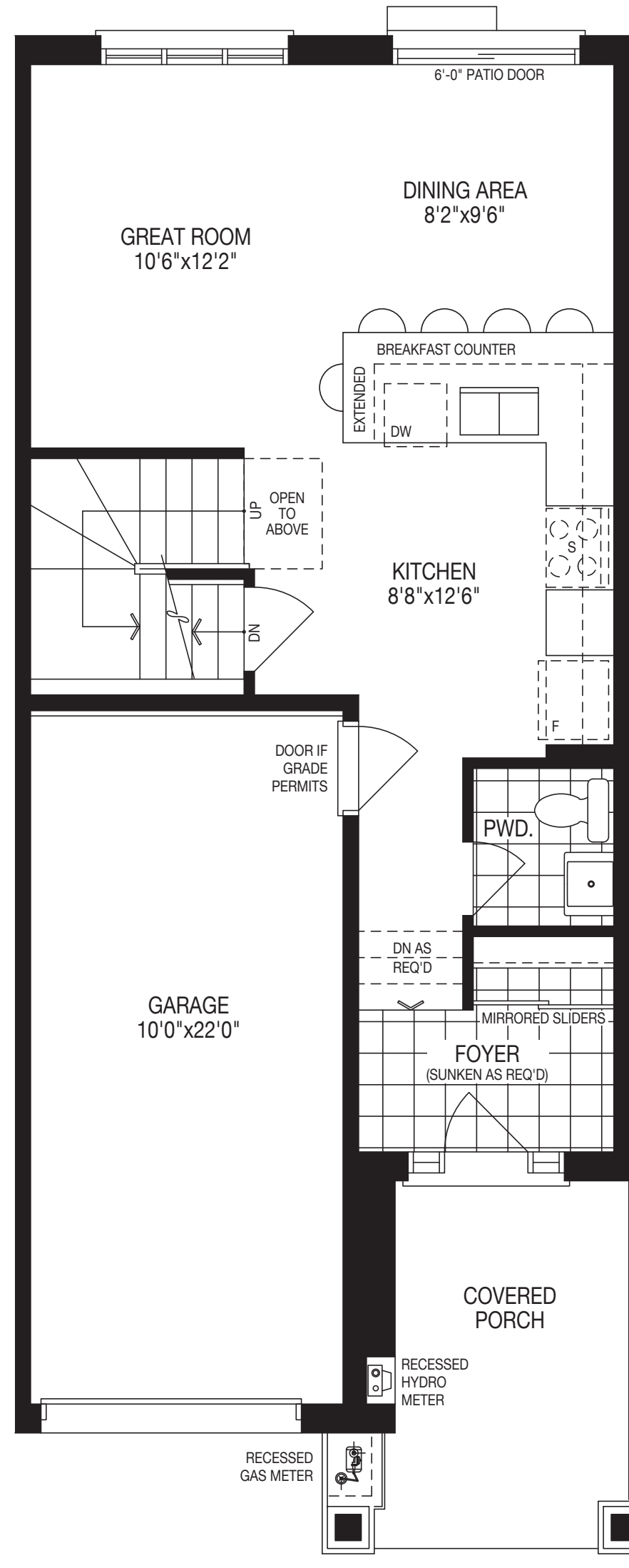
Main Floor ELEVATION A/B
