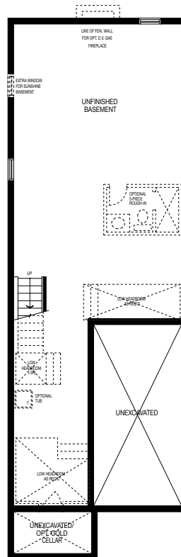
Basement ELEVATION A/B/C/D
