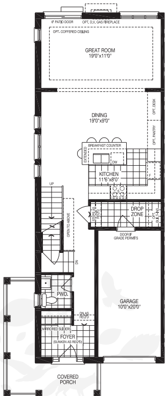
Main Floor CORNER ELEVATION A
